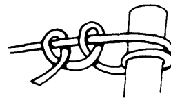
Round turn with two half-hitches.
